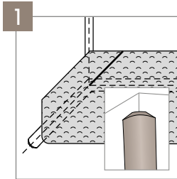
1 Cove former for internal wall angles CA 12 - H204
